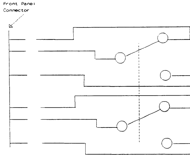
Figure 1: Typical DPDT Relay
