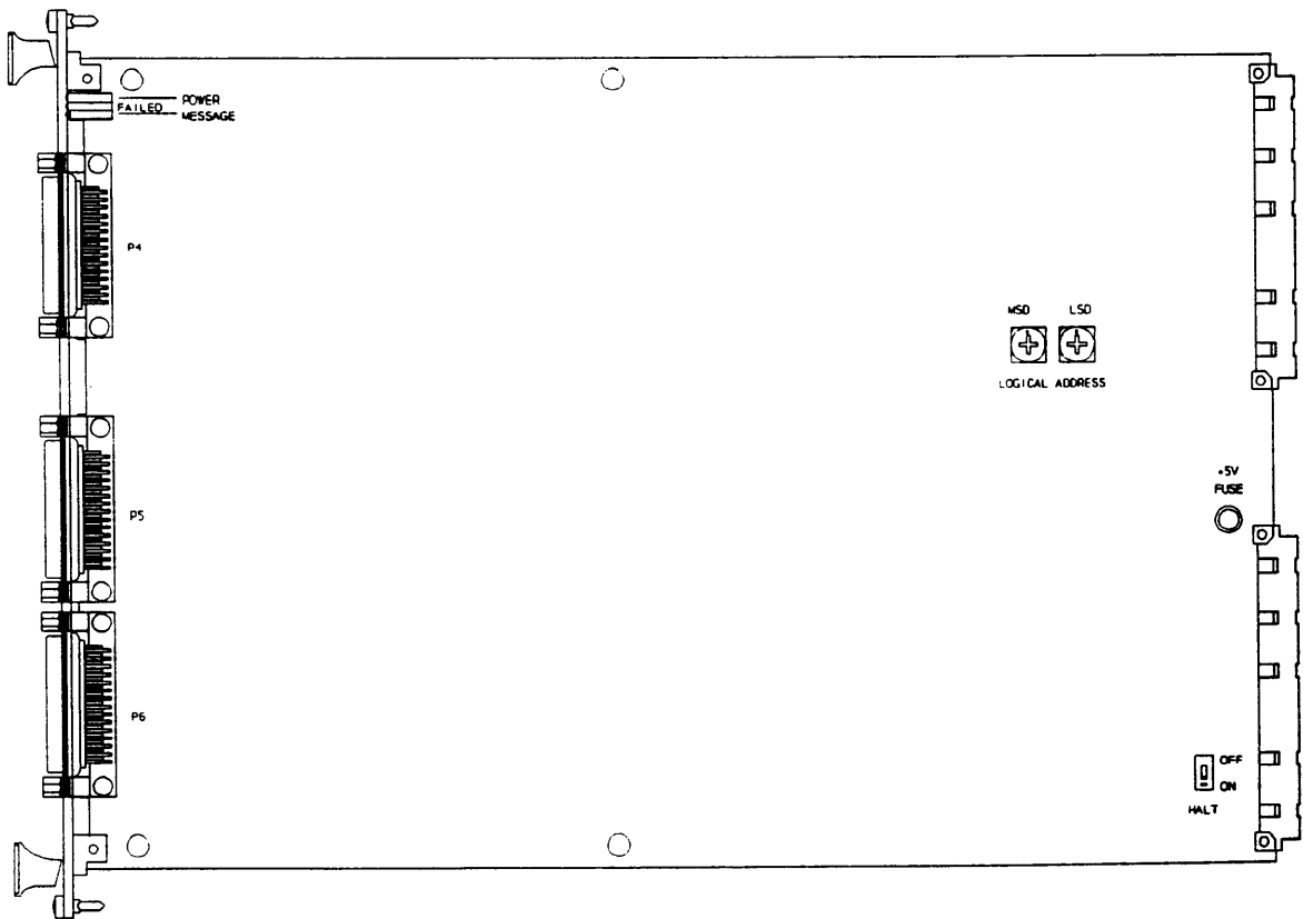
Figure 2: VX4356 Controls and Indicators
